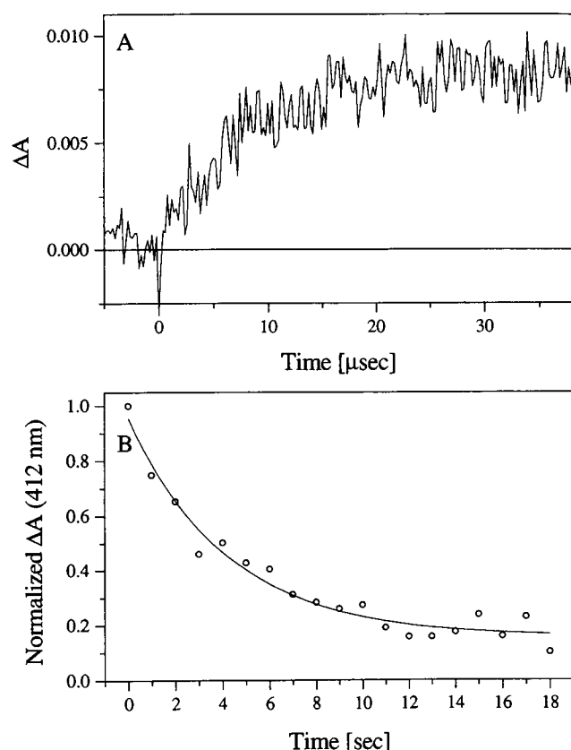
FIGURE 3 Formation and decay kinetics of M' at 67% humidity. (A) Formation of M' detected at 412 nm following irradiation with 532-nm NdYag laser. (B) Decay of M' after excitation with a flash lamp.
