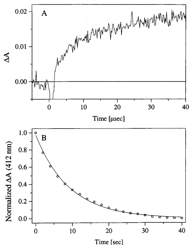
FIGURE 6 Formation and decay kinetics of M' of the D96N mutant at 67% humidity. (A) Formation of M' detected at 412 nm after irradiation with 532-nm NdYag laser. (B) Decay of M' after excitation with a flash lamp.
