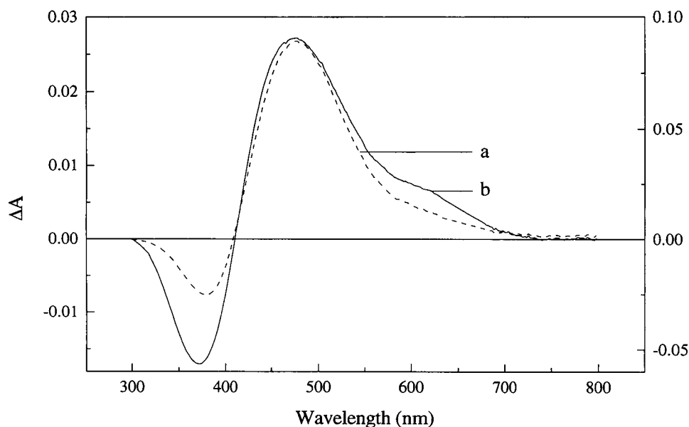
FIGURE 5 Formation of the 570-nm species at low humidity. (a) Difference spectrum between 470 and 390-nm species, following irradiation of 390 species and thermal process for 15 min (right y-axis). (b) Difference spectrum after irradiation of the 470-nm species with 470 nm cutoff filter and thermal process for 15 min (left y-axis).
