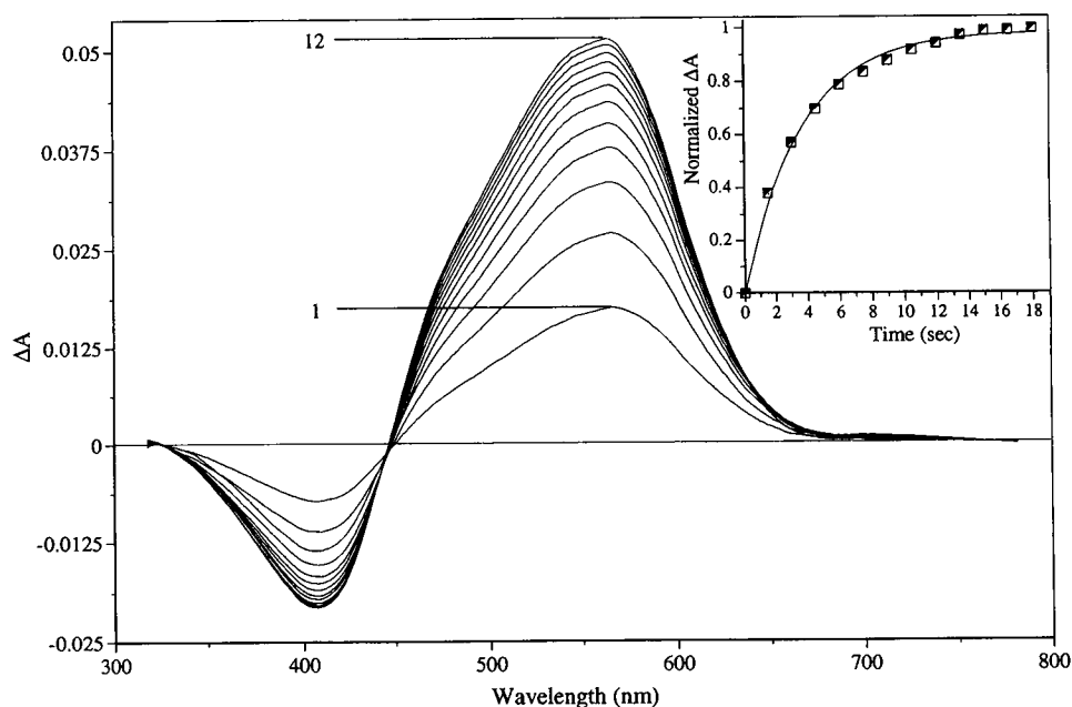
FIGURE 2 Difference absorption of 410-nm species ( M' ) thermal transition to the 570-nm species ( bR' ) following light absorption by bR' . Spectra were taken every 1.5 s, 12 after 18 s. Inset : The best fit (solid line) for the kinetic of bR' reformation from M' based on a monophasic model.
