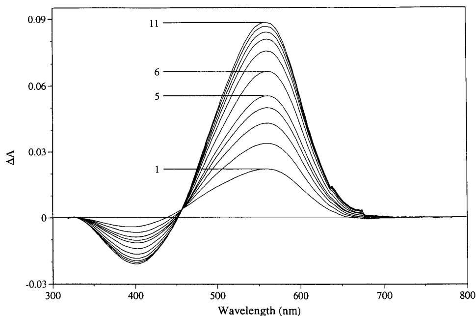
FIGURE 4 Formation of 570-nm species from AbR complex under 51% humidity at pH = 5.5. Difference spectra between 570-nm species and 390-nm species following irradiation of the AbR complex. 1–5 spectra were taken every 30 s, 6 after 240 s, 11 after 14 min (6–11 every 120 s).
