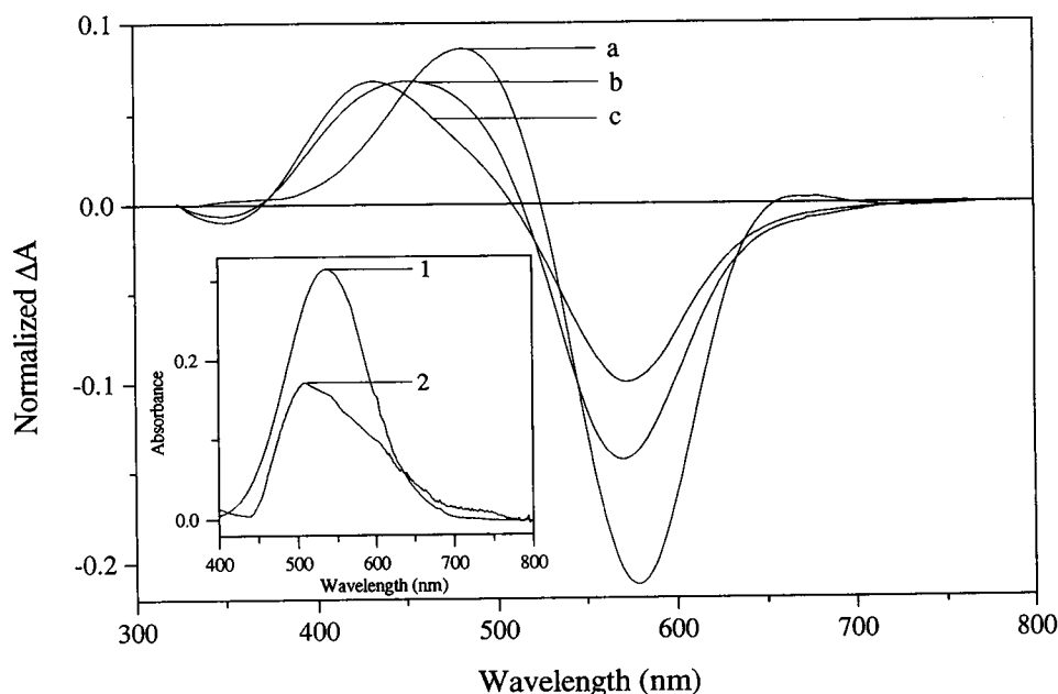
FIGURE 1 Difference absorption spectra of 570 nm to 490 nm or 440 nm transition following dehydration. The dehydration was carried out by applying high vacuum (1 mm Hg). (a) native bacteriorhodopsin; (b) reconstituted 570-nm species under 86% humidity; (c) reconstituted 570-nm species at 51% humidity. Inset: (1) Absorption of native bacteriorhodopsin following dehydration. (2) Absorption of reconstituted 570-nm species at 51% humidity following dehydration.
