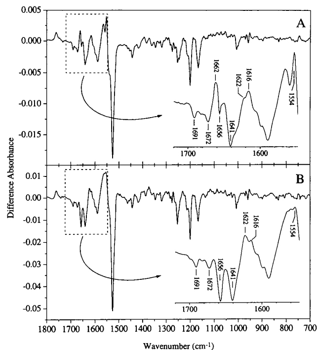
FIGURE 7 Difference FTIR spectra of M'/bR' spectra transition. (A) M'/bR' at 67% humidity; (B) M/bR difference spectrum of the same sample obtained after an increase in the humidity to 100%. Positive peaks are due to M' or M species and negative peaks are due to bR and bR'. Spectra were taken at 250 K. The sample was obtained by illumination of 9- cis retinal-bacterioopsin complex (AbR) under 67% humidity, followed by thermal conversion under the same humidity.
